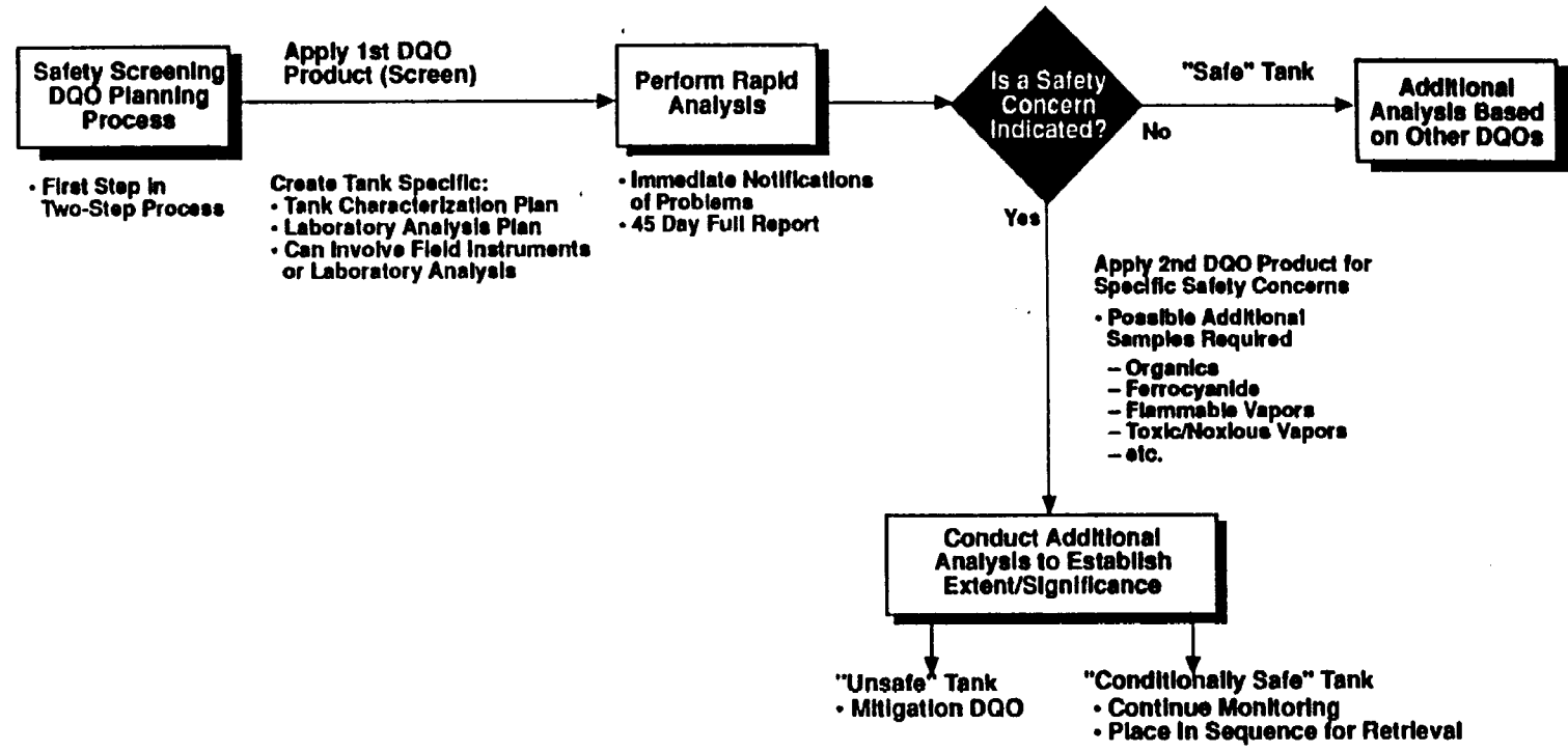
Figure 4. Logic Flow Addressing Safety Concerns.
